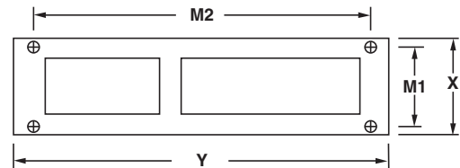
Mold Mounting Footprint
