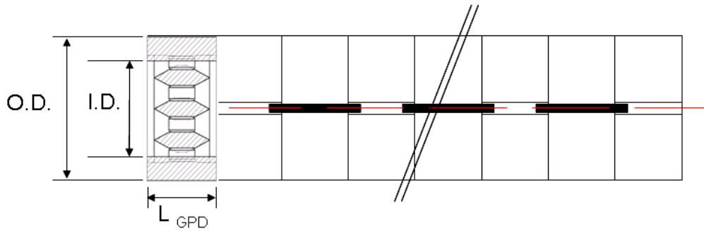
View of GPD showing the installation
