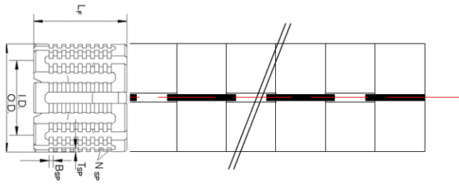
View of SMF-Filter showing main dimensions
